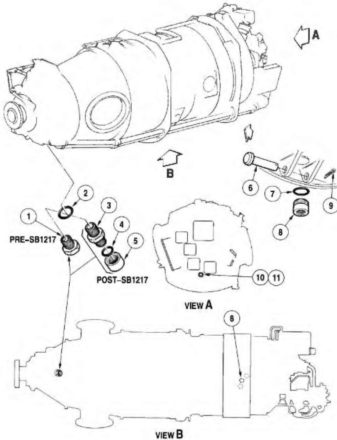
Figure Location of Drain plugs
