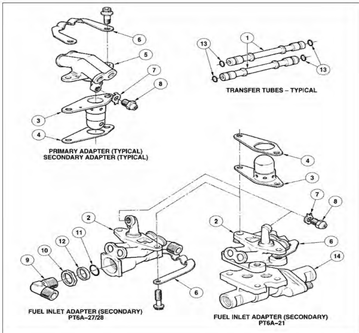
Figure 202 - Removal/ Installation of Fuel Manifold Adapter
