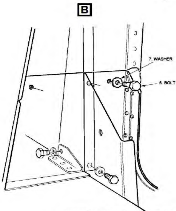
Powerplant - Removal / Installation - Engine Bulkheads Figure 407
