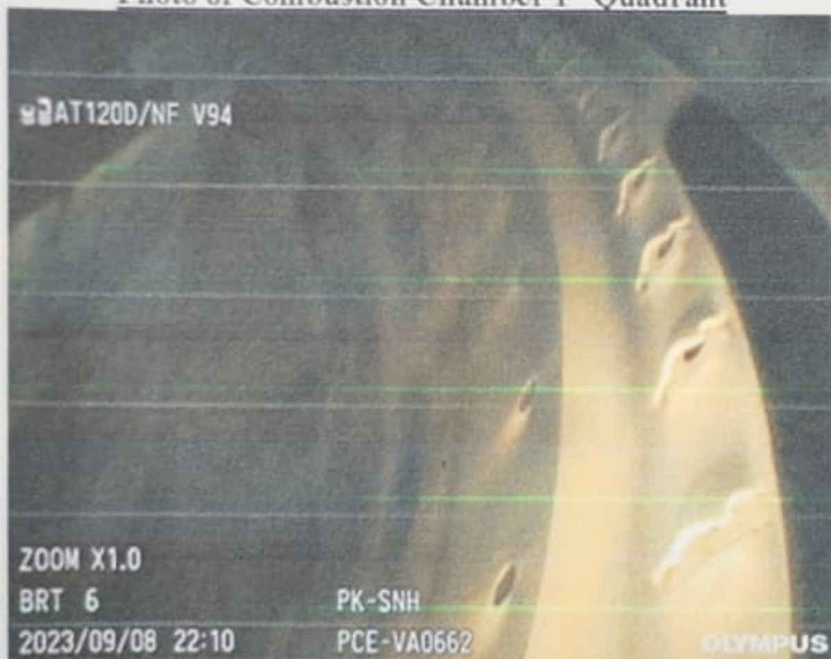
Photo of Combustion Chamber 1 st Quadrant
