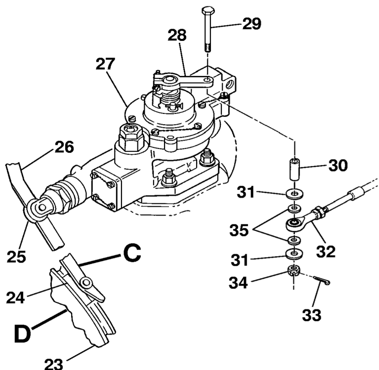
DETAIL B PROPELLER GOVERNOR
